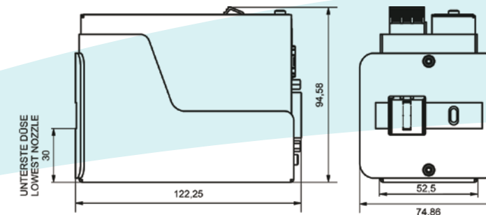
Dimension drawing technical data
